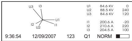
Example phasor display
