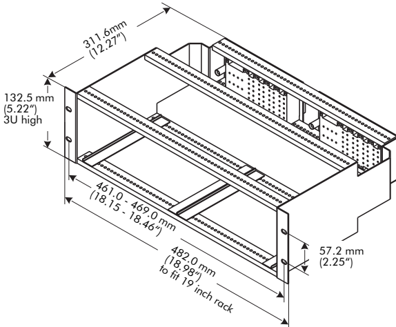
Front of Rack View
