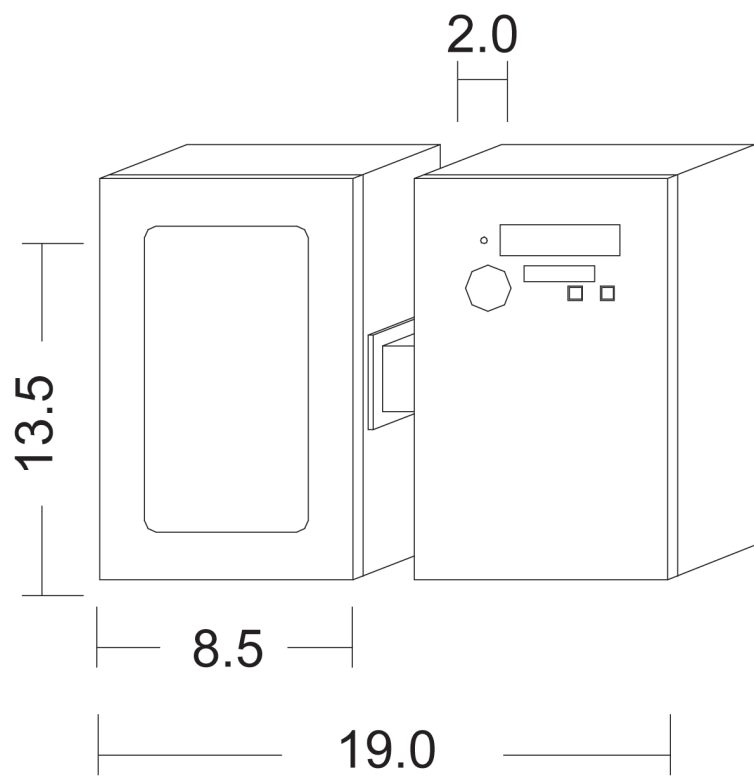
MiniCloset-5 Dimensions (Choose the orientation best suited for the installation site.)
